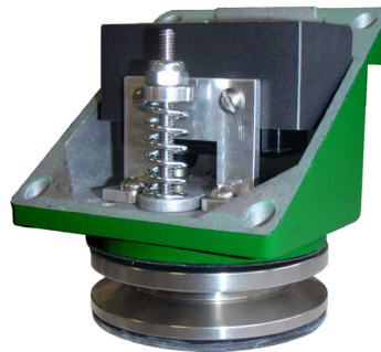
Solon Sanitary Connection Pressure Switch
